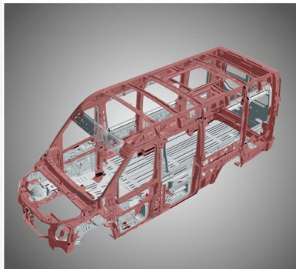
Frontal Crash Compliant Monocoque Structure
