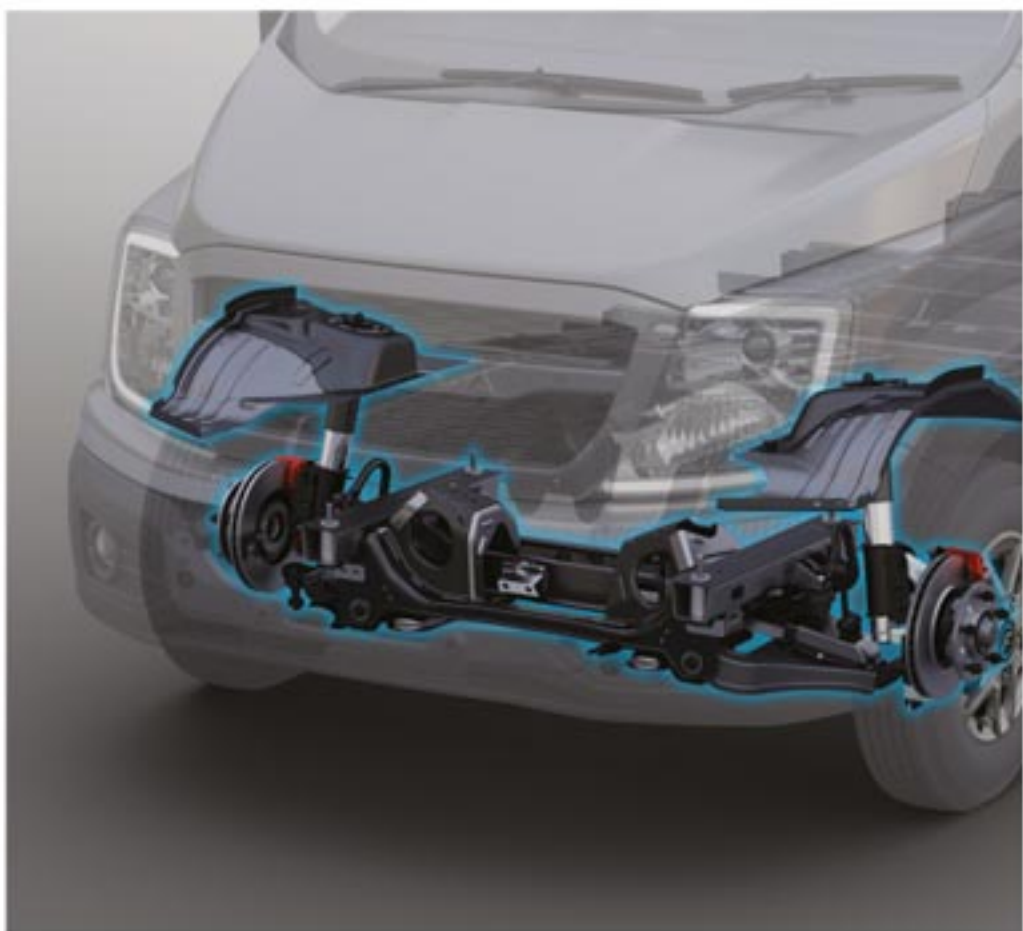
Independent Front Suspension & All Wheel Disc Brakes
